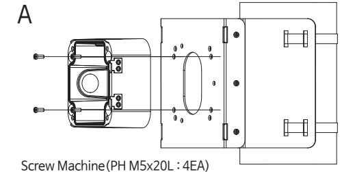
Screw Machine (PH M5x20L : 4EA)
